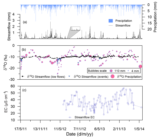
Figure 2. (a) Hourly precipitation and unit area streamflow; (b) \delta^{18}\text{O} isotopic composition in precipitation and streamflow for 3 years (May 2011 to May 2014); and (c) electrical conductivity for 2 years (May 2012 to May 2014) at the catchment outlet (M8; see location in Fig. 2). The size of the bubbles in plot (b) indicates the relative cumulative rainfall in millimeters for each collected sample.
