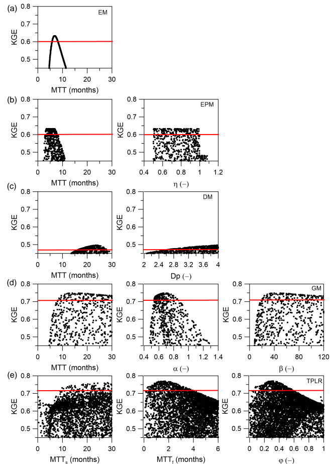
Figure 4. Monte Carlo simulations of the fitted parameters of the five lumped parameter models used to simulate the \delta^{18}\text{O} streamflow composition at the outlet of the basin (M8). (a) EM; (b) EPM; (c) DM; (d) GM; and (e) TPLR. The (–) symbol on the x axes denotes that the fitting parameter is dimensionless. Horizontal red lines indicate the threshold of behavioral solutions (at least 0.95 of maximum KGE).
