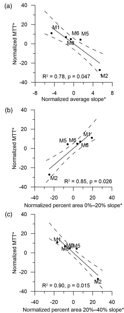
Figure 6. Correlations between mean transit time (MTT) and topographic indexes of the catchments: (a) average catchment slope; (b) catchment area with slopes between 0 and 20 %; and (c) catchment area with slopes between 20 and 40 %. Catchments M3 and M4 (additional spring water source; see Fig. 1) and M7 (at a flat hilltop disconnected from the hillslopes) are not included in the regressions. Solid lines are linear regressions and dashed lines are the 90 % confidence intervals of the regressions. * indicates variables are normalized by their means.
