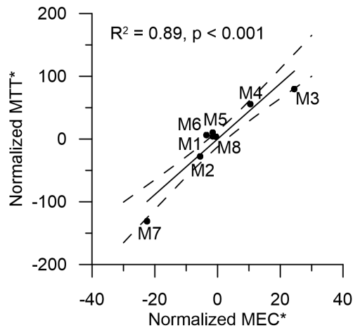
Figure 7. Correlation between mean transit time (MTT) and mean electrical conductivity (MEC) for weekly measurements of stream-water samples collected during 3 years (June 2012 to June 2015). The solid line is the linear regression and the dashed lines are the 90 % confidence intervals of the regression. * indicates variables are normalized by their means.
