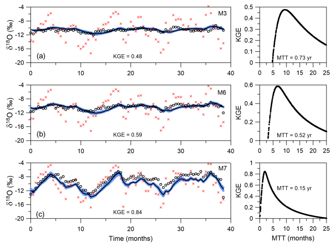
Figure 5. Fitted results and Monte Carlo simulations of the fitted parameters of the exponential model (EM) used to simulate the \delta^{18}\text{O} streamflow composition in the catchments: (a) M3; (b) M6; and (c) M7. The open circles represent the observed isotopic composition in streamflow; the red crosses represent the isotopic composition in precipitation; the black line represents the best simulated isotopic composition in streamflow according to the KGE objective function; and the blue shaded area corresponds to the 5–95 % confidence limits of the possible solutions from the MTT fitting parameters within the range of behavioral solutions, i.e., solutions that yield at least 95 % KGE. Panels on the right represent the explored parameter range for the MTT parameter and the KGEs associated with each of them.
